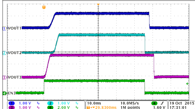
图 9-37. Automatic Power Sequencing, MODE = HIGH, EN1 = LOW, EN2 = HIGH
