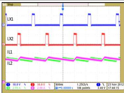
Figure 40. Steady State of Current Share Mode Operation ( I_O = 10\text{ A} )
