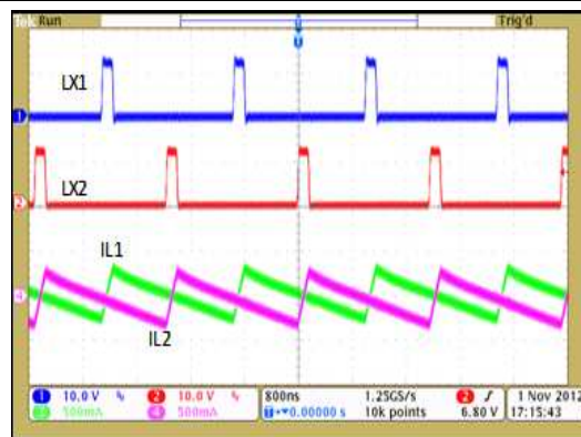
Figure 39. Steady State of Current Share Mode Operation ( I_O = 0\text{ A} )
