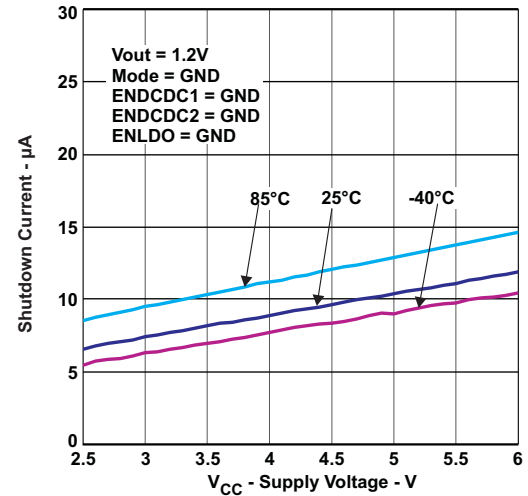
Figure 20. Shutdown Current
