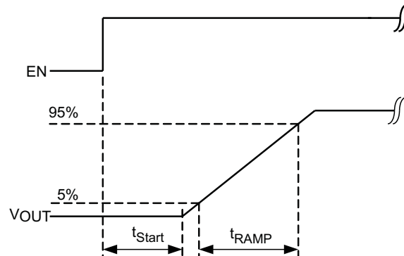
Figure 21. Soft Start
