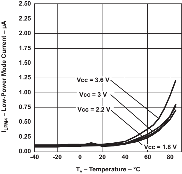
图 3-5. LPM4 Current vs Temperature
