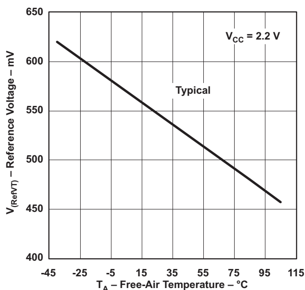
图 3-22. V (RefVT) vs Temperature, V CC = 2.2 V
