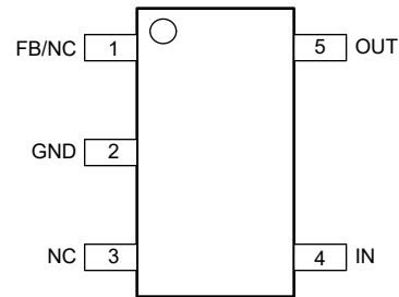
图 4-2. DCK Package, 5-Pin SC70 (Top View)
