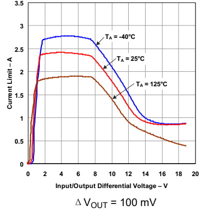
图 5-14. Current Limit vs Input/Output Differential Voltage
