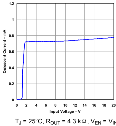
图 5-5. Quiescent Current vs Input Voltage
