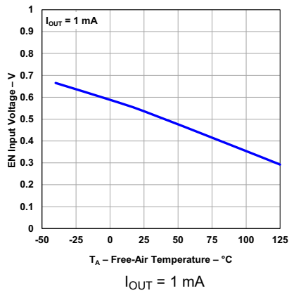
图 5-11. EN Threshold (Off to On) vs Temperature
