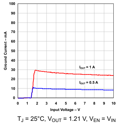
图 5-6. Ground Current vs Input Voltage
