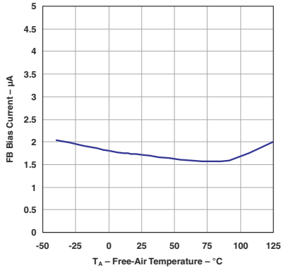
图 5-13. Fb Bias Current vs Temperature
