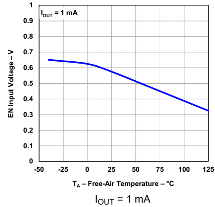
图 5-12. EN Threshold (On to Off) vs Temperature
