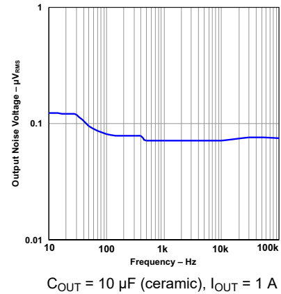
图 5-20. Output Noise Voltage vs Frequency
