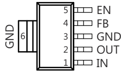
图 4-1. DCQ Package, 6-Pin SOT-223 (Top View)
