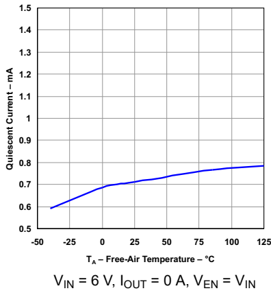
图 5-3. Quiescent Current vs Temperature
