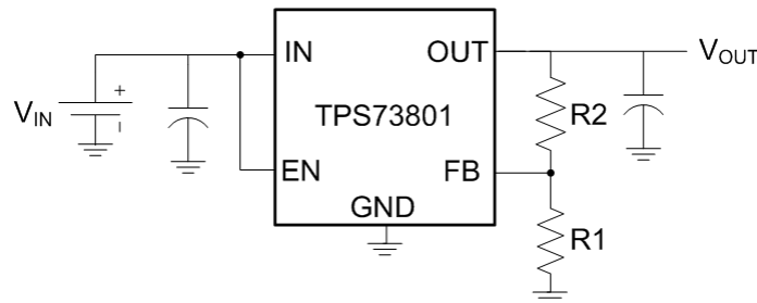
图 6-1. Adjustable Operation
