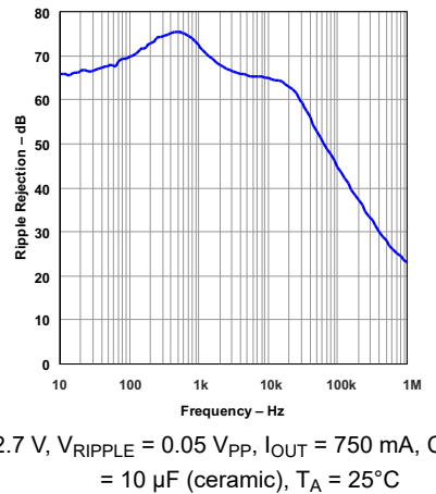
图 5-18. Ripple Rejection vs Frequency
