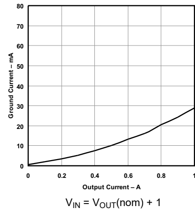
图 5-8. Ground Current vs Output Current
