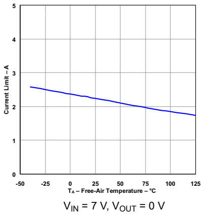
图 5-15. Current Limit vs Temperature
