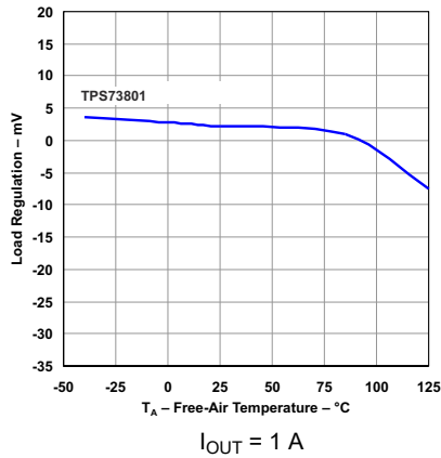
图 5-19. Load Regulation vs Temperature
