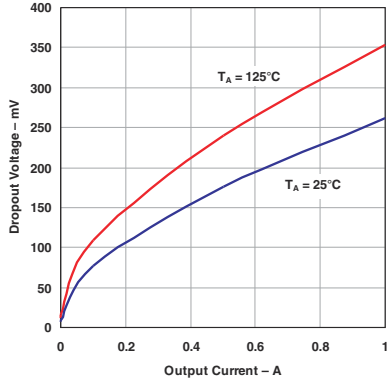
图 5-1. Dropout Voltage vs Output Current
