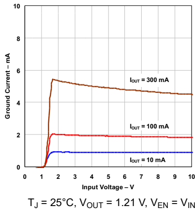
图 5-7. Ground Current vs Input Voltage
