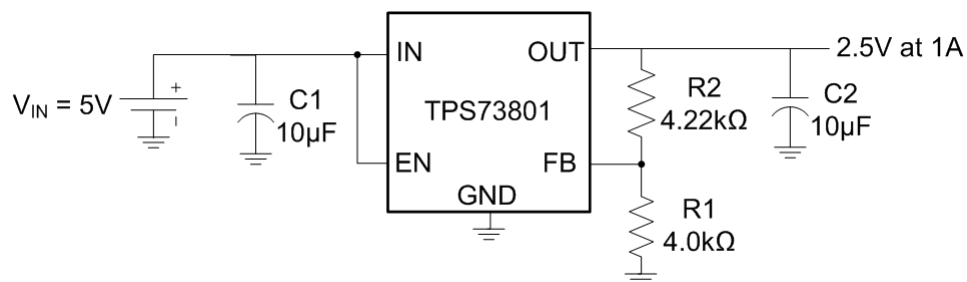
图 7-1. Adjustable Output Voltage Operation
