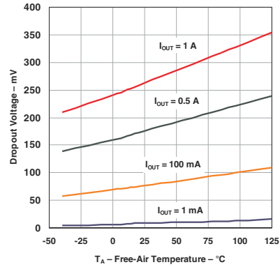
图 5-2. Dropout Voltage vs Temperature
