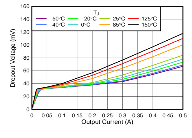
图 4. 3.3-V Dropout Voltage vs I_{OUT}
