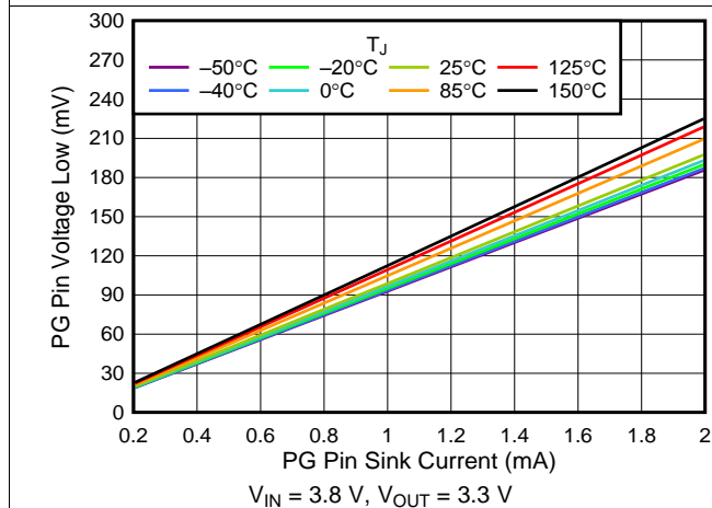
图 17. V OL (P G ) vs P G Pin Sink Current
