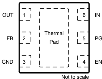
DRV Package 6-Pin Adjustable WSON Top View
