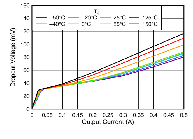
图 6. 5.5-V Dropout Voltage vs I_{OUT}
