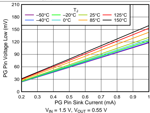
图 18. V OL (P G ) vs P G Pin Sink Current
