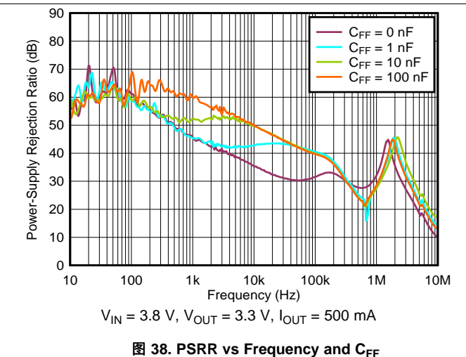
图 38. PSRR vs Frequency and C_{FF}
