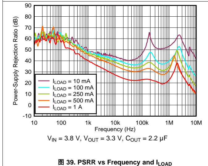
图 39. PSRR vs Frequency and I_{LOAD}
