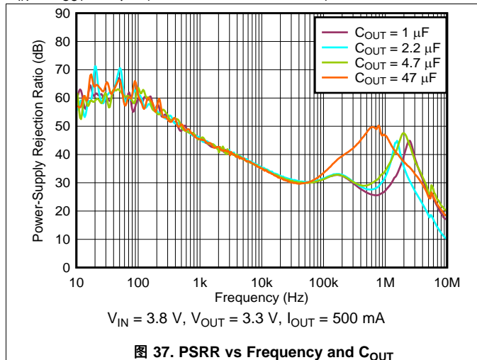
图 37. PSRR vs Frequency and C_{OUT}
