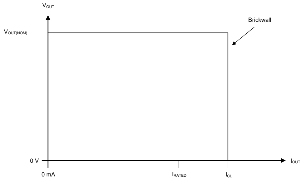
Figure 6-4. Current Limit
