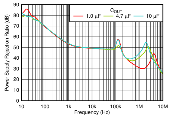
图 6-68. PSRR vs Frequency and C_{OUT}
