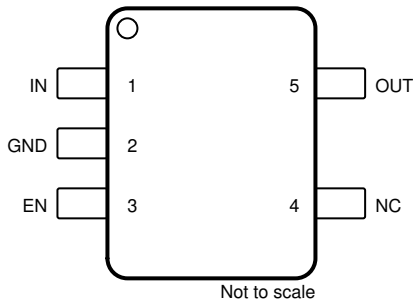
图 5-1. DBV Package (Fixed), 5-Pin SOT-23, Top View
