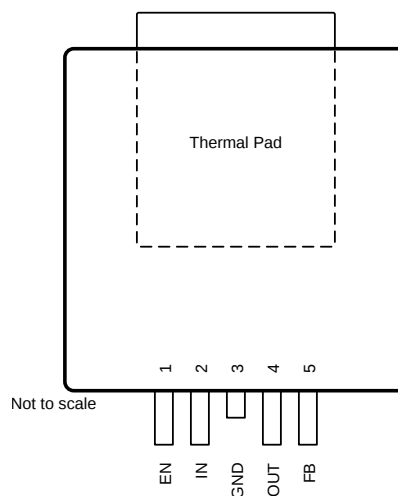
图 5-6. KVV Package (Adjustable), 5-Pin TO-252 (Top View)
