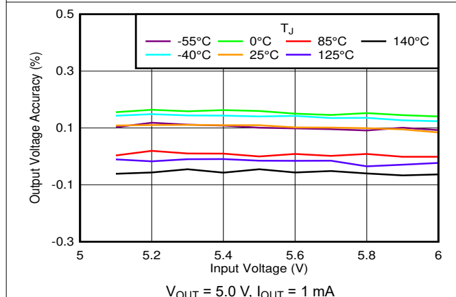
图 6-29. Output Accuracy vs V_{IN} and Temperature
