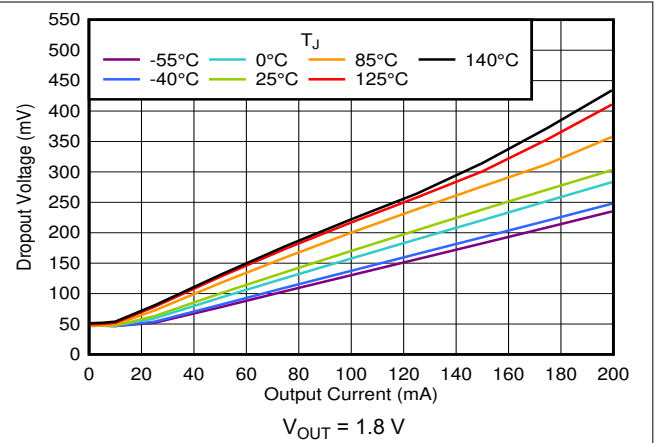
图 6-32. Dropout vs I_{OUT} and Temperature
