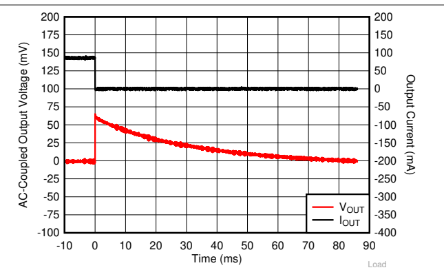
图 6-18. I_{OUT} Transient From 100 mA to 0 mA
