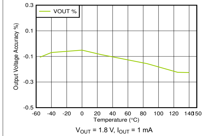
图 6-27. Output Accuracy vs Temperature
