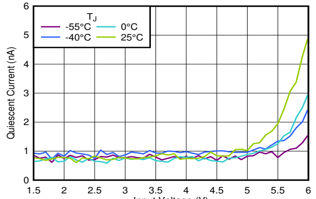
图 6-8. I_Q in Dropout vs V_{IN} and Temperature
