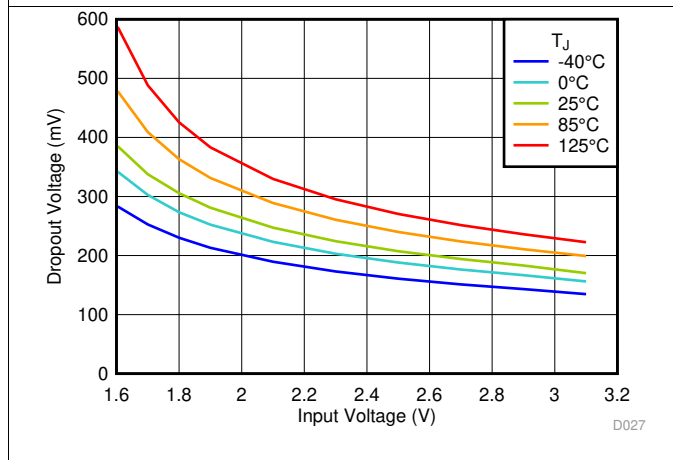
图 23. Dropout vs V_{IN} and Temperature
