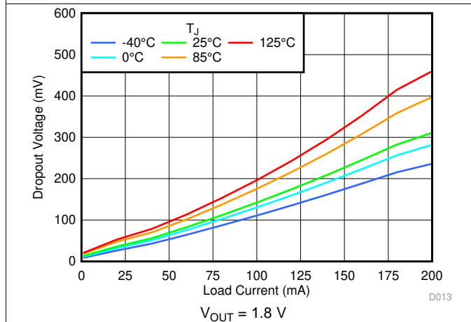
图 21. Dropout vs I_{OUT} and Temperature
