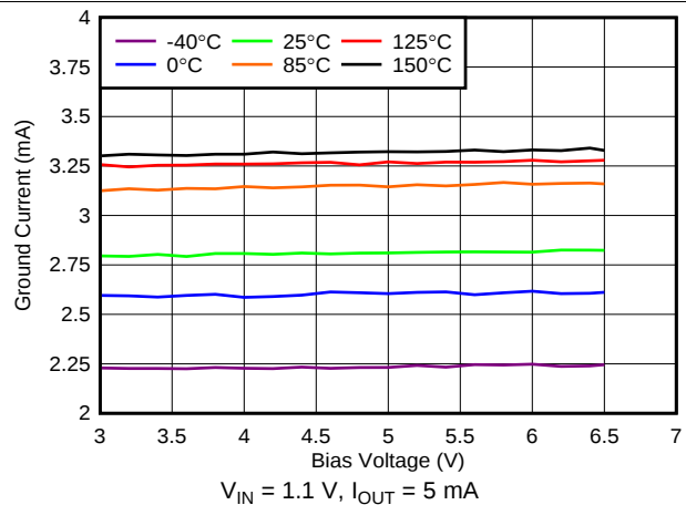
图 28. Ground Current vs Bias Voltage
