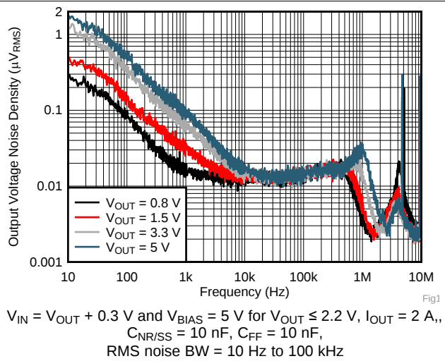
图 10. Output Noise vs Frequency and V_{OUT}
