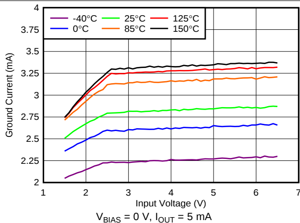
图 27. Ground Current vs Input Voltage
