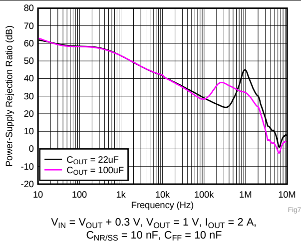
图 7. PSRR vs Frequency and C_{OUT}
