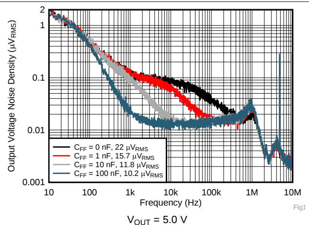
图 49. Noise vs Frequency and C_{FF}
