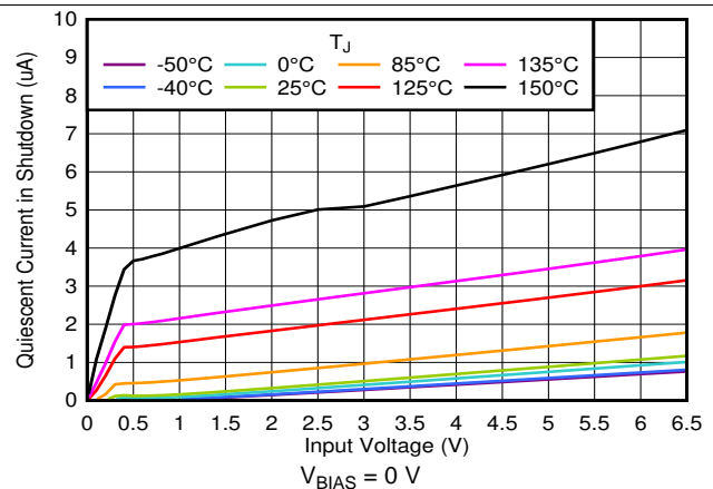
图 30. Shutdown Current vs Input Voltage
