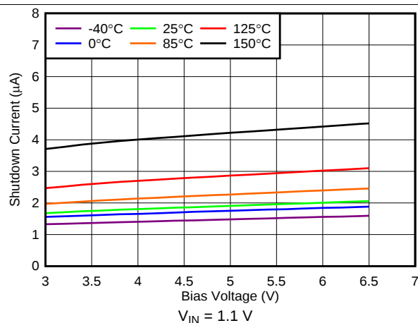
图 30. Shutdown Current vs Bias Voltage
