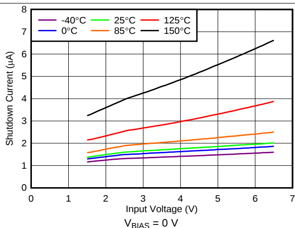
图 29. Shutdown Current vs Input Voltage
