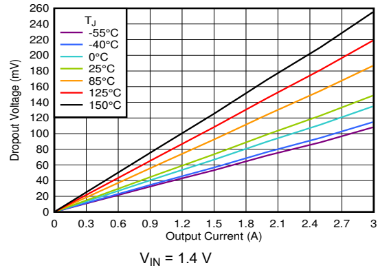
图 6-68. Dropout Voltage vs I_{OUT} Without Bias
