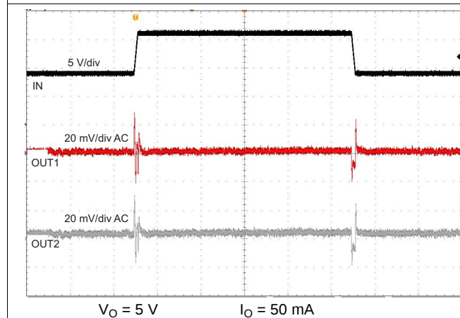
图 15. 9-V to 16-V Line Transient (1 V/μs)
