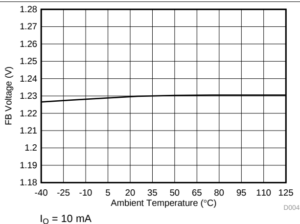
图 6. FB Voltage vs Ambient Temperature
