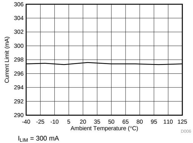
图 8. Current Limit vs Ambient Temperature
