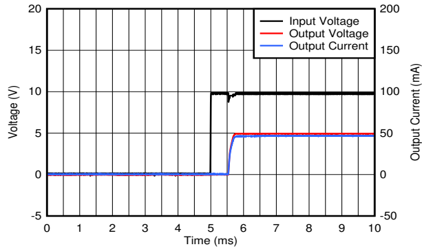
图 8-5. Power-Up Waveform
