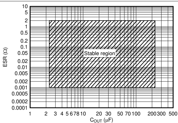
图 6-31. Stability ESR vs C_{OUT}
