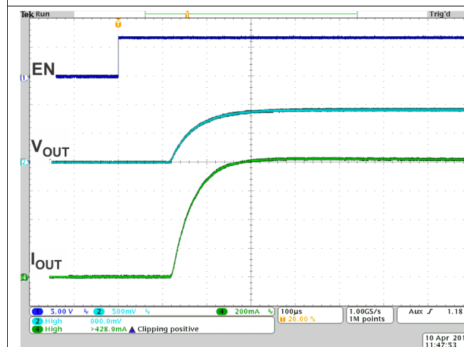
Figure 26. Startup for TPS8268090 (Vin = 5V, Vout = 0.9V)
