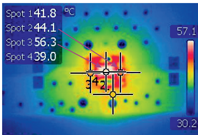
Figure 31. V_{IN}=5V , V_{OUT}=1.05V , I_{OUT}=1.2A 466mW Power Dissipation
