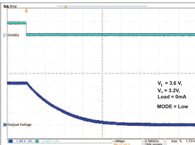
Figure 26. TPS82699 Shut-Down
