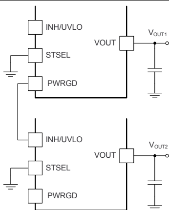
Figure 30. Sequencing Schematic
