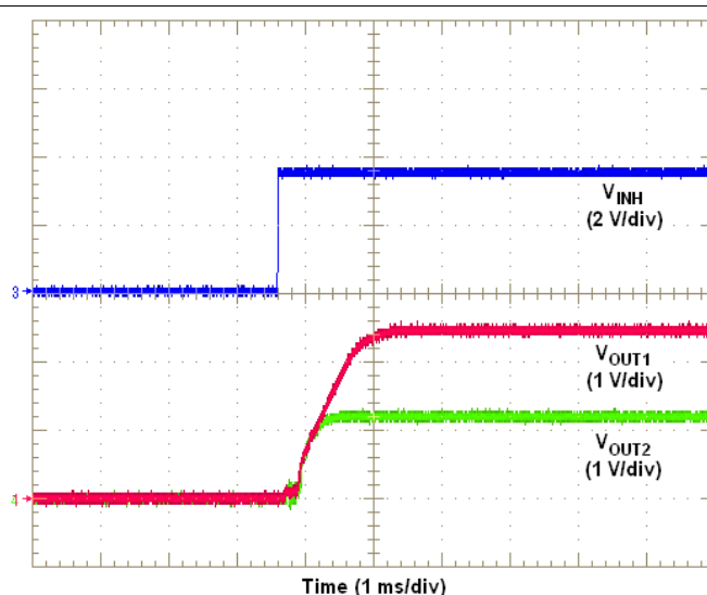
Figure 33. Simultaneous Tracking Waveforms
