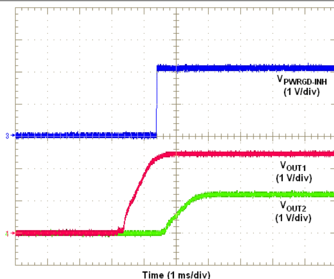
Figure 31. Sequencing Waveforms
