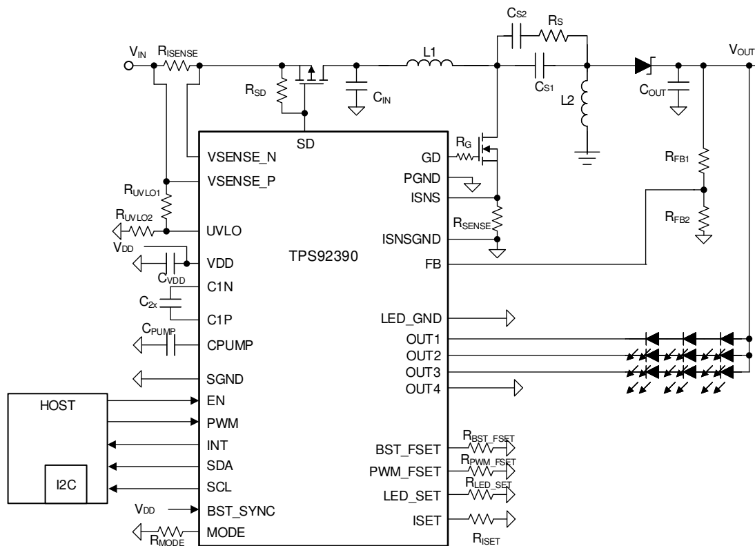
图 8-6. SEPIC 模式 with Three LEDs in Series
