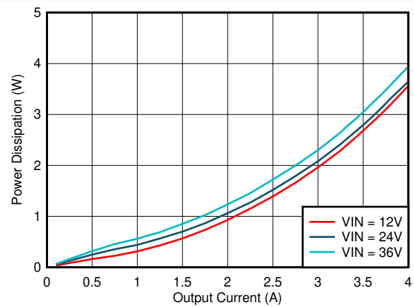
图 6-2. Power Dissipation V_{OUT} = 3.3 \text{ V} , T_A = 25^\circ\text{C}
