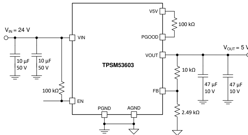
图 8-1. TPSM53603 Typical Schematic
