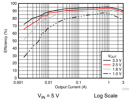
图 6-2. Efficiency versus Output Current
