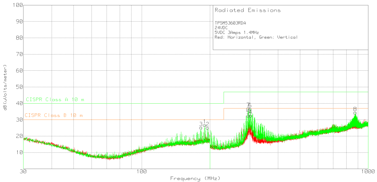
图 10-5. Radiated Emissions 24-V Input, 5-V Output, 3-A Load
