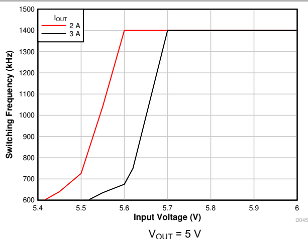
图 7-10. Frequency Foldback
