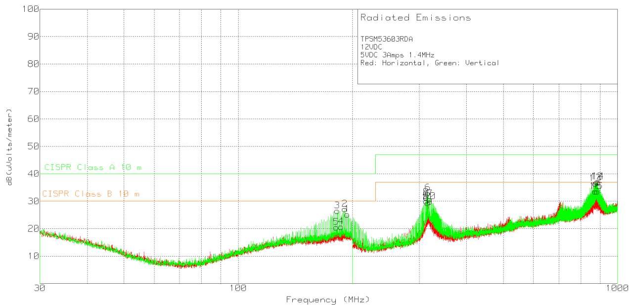
图 10-6. Radiated Emissions 12-V Input, 5-V Output, 3-A Load
