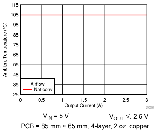
图 6-5. Safe Operating Area
