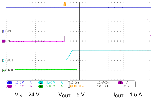
图 9-2. Start-up Waveforms
