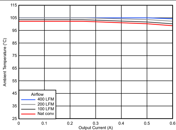
图 6-19. Safe Operating Area ( V_{OUT} = 12\text{ V} )
