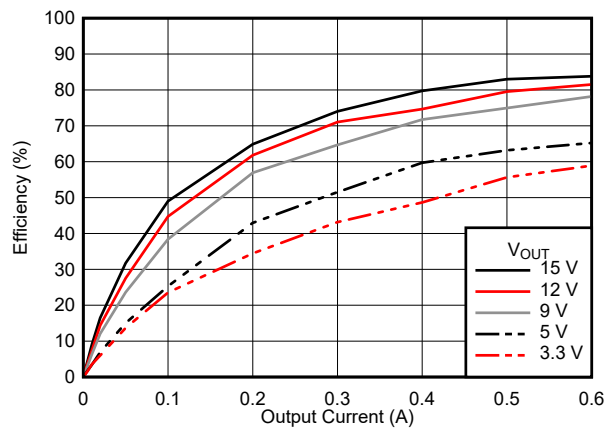
图 6-15. Efficiency
