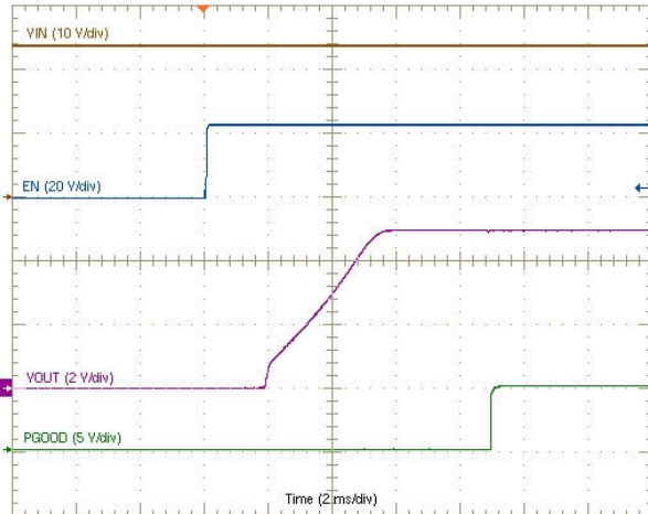
图 8-2. Start-Up Waveforms
