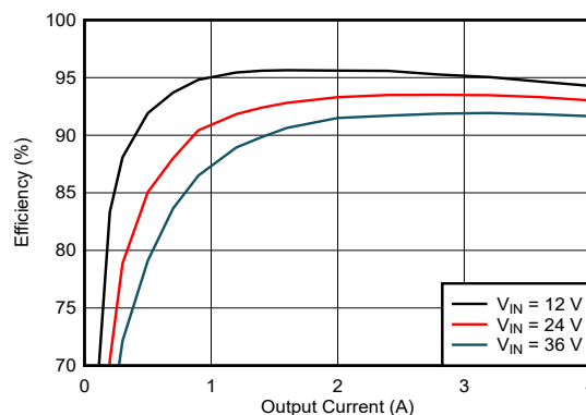
典型效率 ( V_{OUT} = 5V , F_{SW} = 1MHz )
