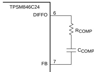
图 14. Compensation Components
