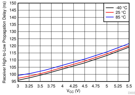
图 5-3. Receiver Path High-to-Low Propagation Delay vs T_A and Supply Voltage (RGT Package)
