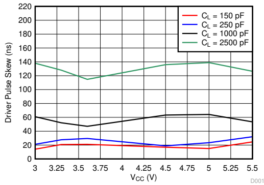
图 5-1. Driver Pulse Skew vs Load Capacitance and Supply Voltage at T_A = 25\text{ }^{\circ}\text{C} (RGT Package)
