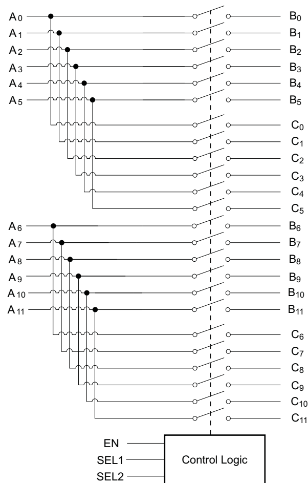
Figure 2. LOGIC DIAGRAM
