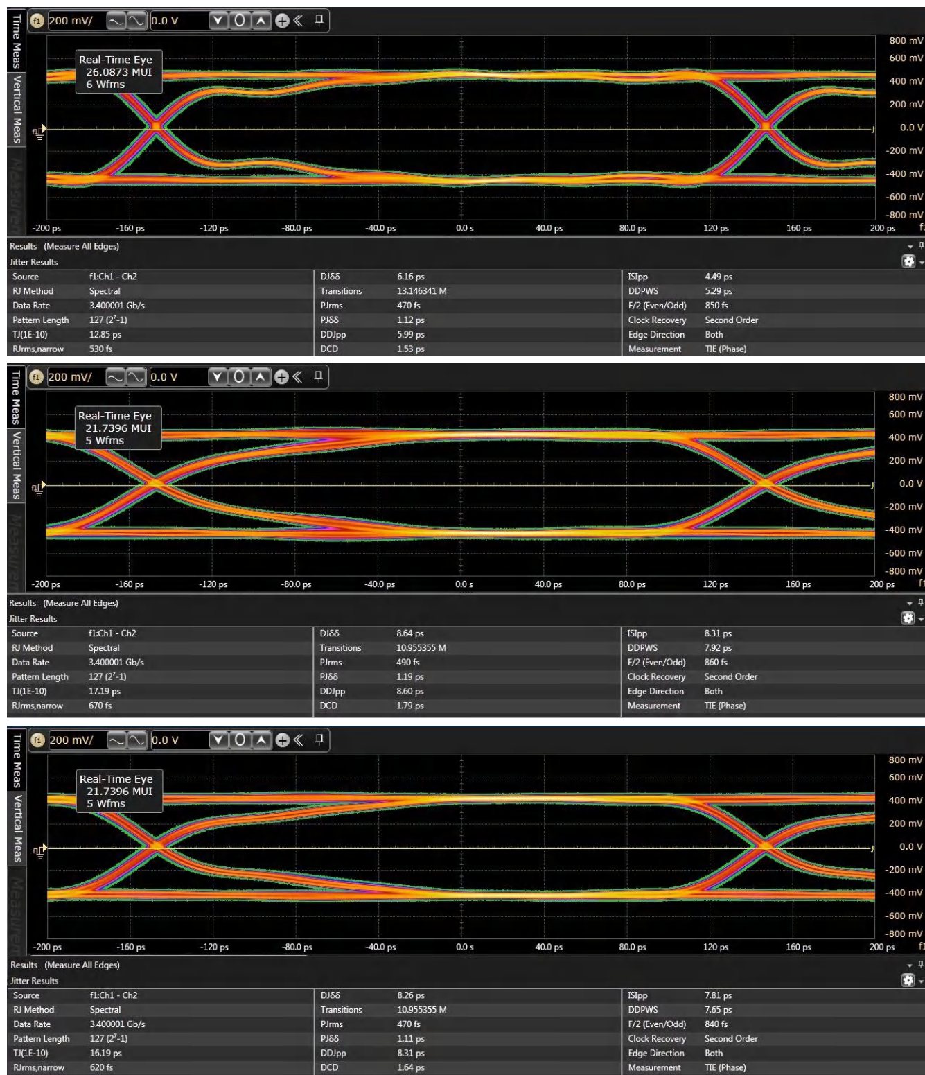
图 6-5. Typical eye diagrams at 3.4 Gbps. Top: baseline calibration setup. Middle: through TS3DV642-Q1 Port A. Bottom: through TS3DV642-Q1 Port B.
