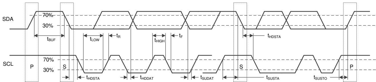
图 2. I²C Timing Diagram Definitions
