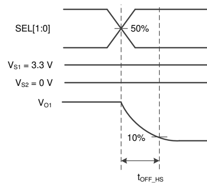
图 15. Turn-ON time ( t_{ON} ) and Turn-OFF time ( t_{OFF} ) for High-Speed Data Paths
