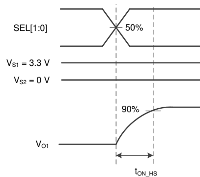
图 15. Turn-ON time ( t_{ON} ) and Turn-OFF time ( t_{OFF} ) for High-Speed Data Paths
