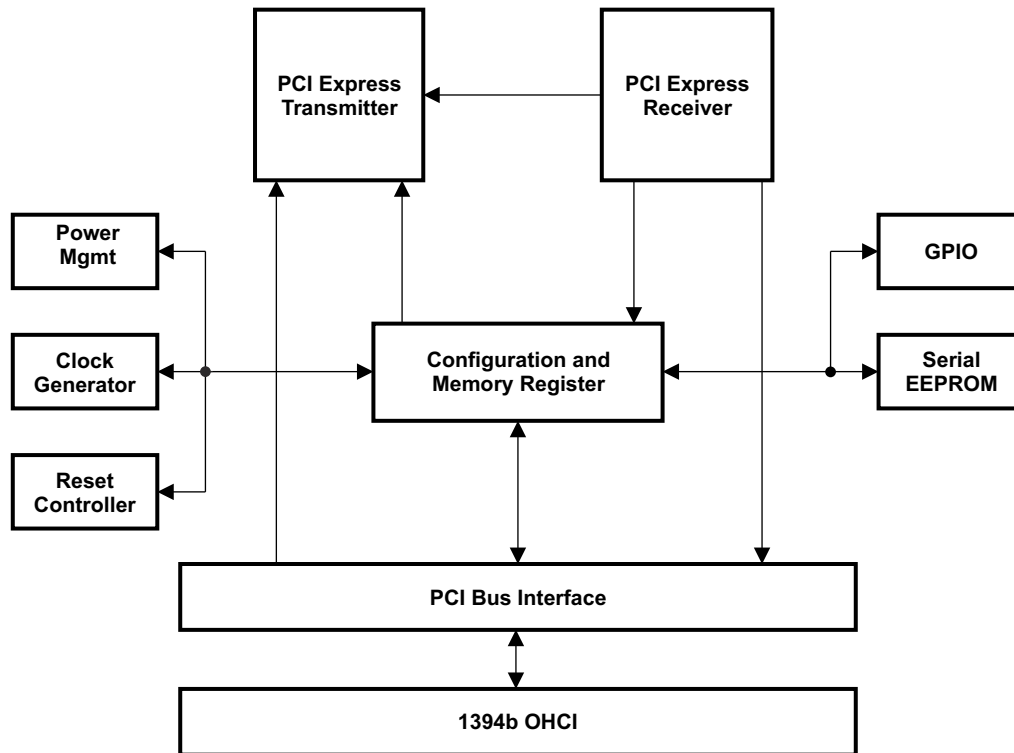
图 10-1. TSB82AF15-EP Block Diagram
