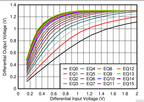
图 6-5. USB TX Linearity Curves at 5 GHz
