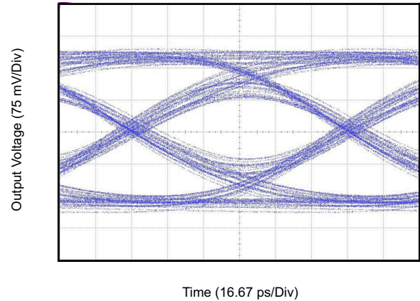
图 6-10. USB 3.1 Gen2 Eye-Pattern Performance with 12-inch Input PCB Trace at 10 Gbps
