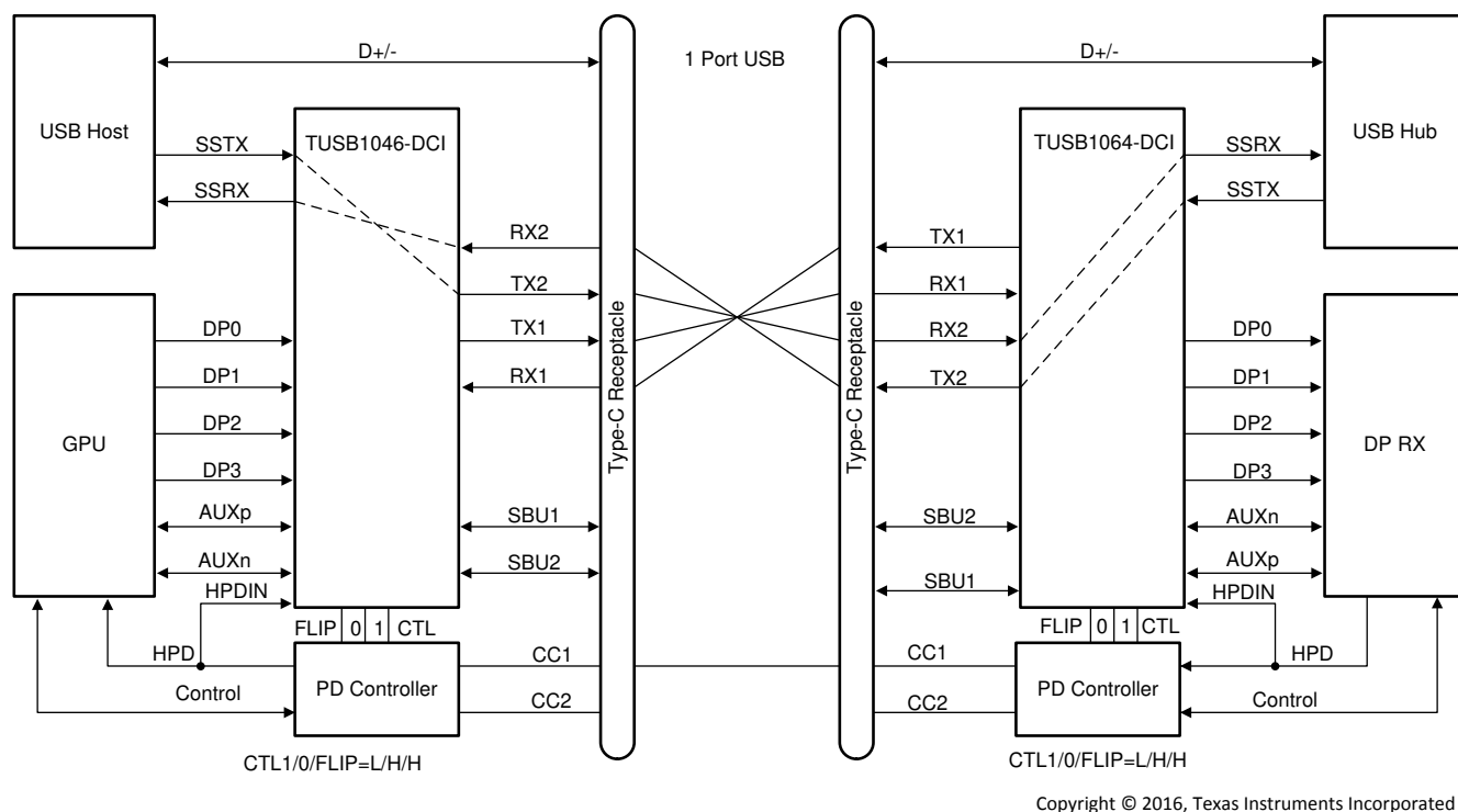
图 8-5. USB3.1 Only - With Flip (CTL1 = L, CTL0 = H, FLIP = H)
