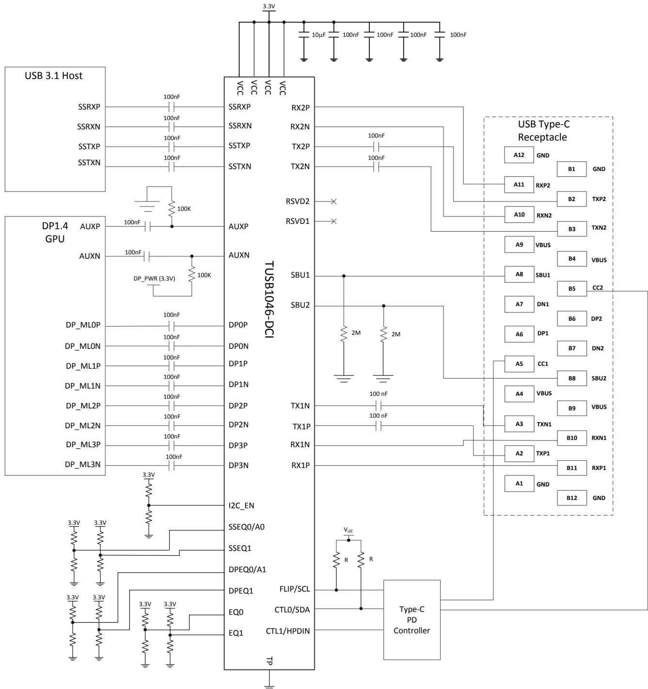
图 8-2. Application Circuit
