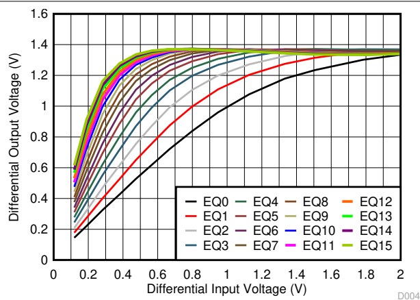
图 6-4. DisplayPort Linearity Curves at 4.05 GHz
