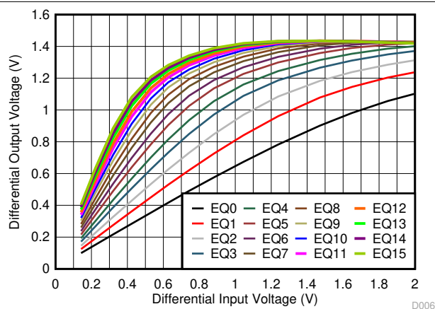
图 6-6. USB RX Linearity Curves at 5 GHz
