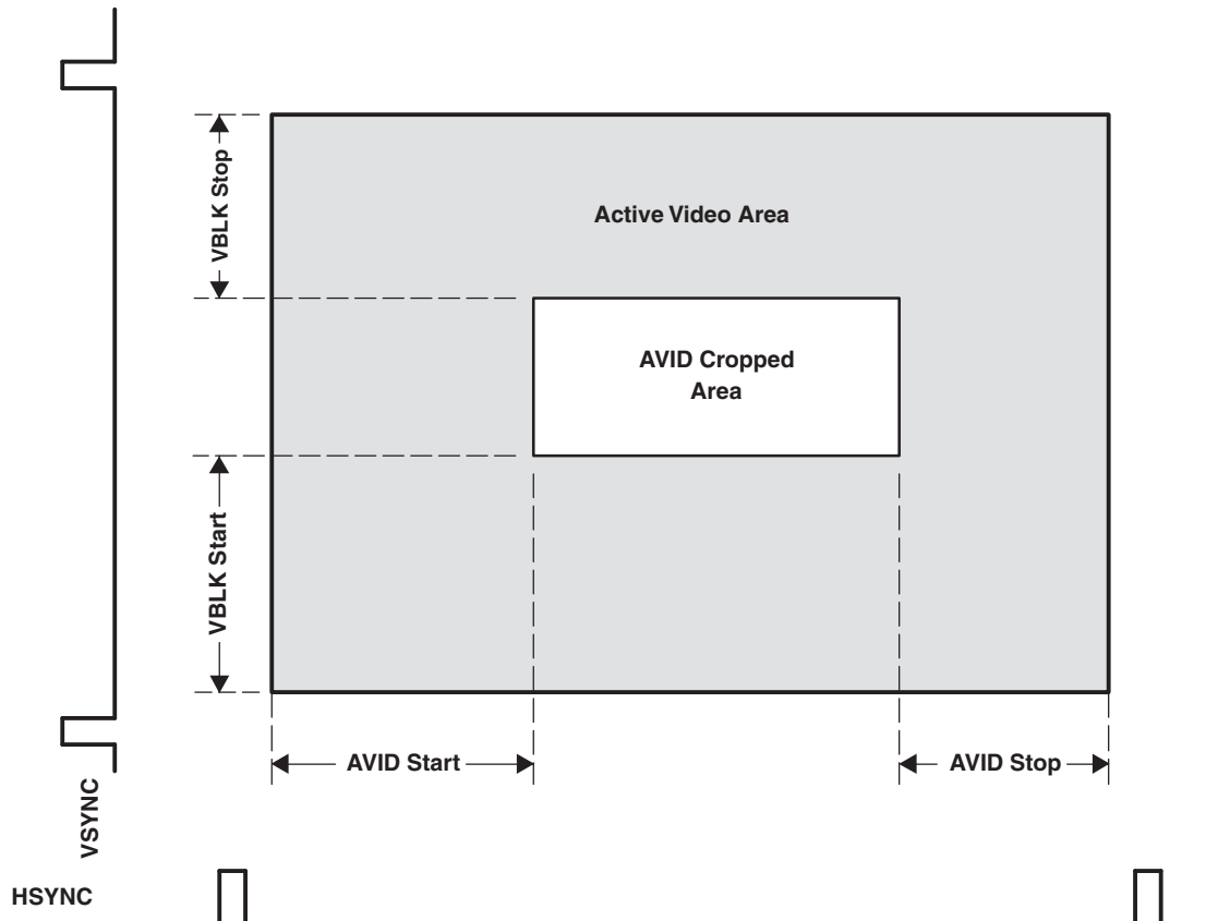
Figure 3-7. AVID Application
