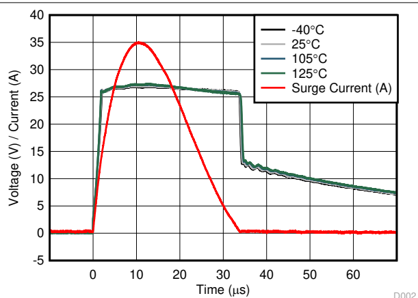
图 7-2. Surge Response at 35 A Across Temperature
