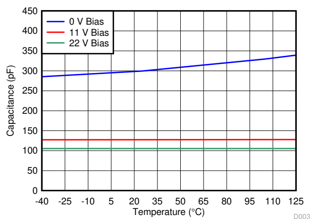
图 7-3. Capacitance vs Temperature Across Bias
