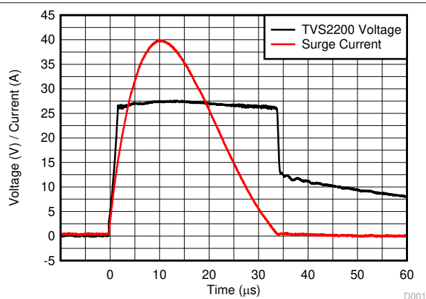
图 7-1. Surge Response at 40 A
