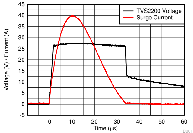
图 9-2. TVS2200 Surge Response at 40 A
