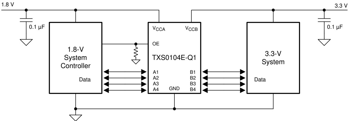
图 8-1. Application Schematic
