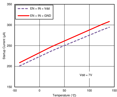
图 6-6. Start-Up Current vs Temperature
