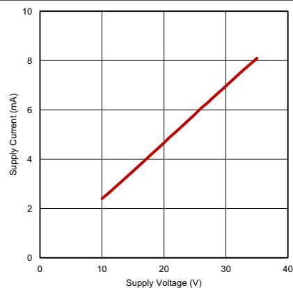
图 6-17. Operating Supply Current vs Supply Voltage (Output Switching)
