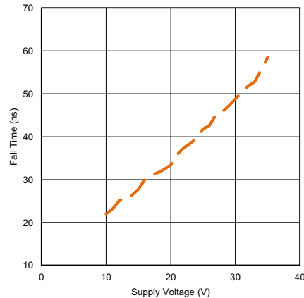
图 6-19. Fall Time vs Supply Voltage
