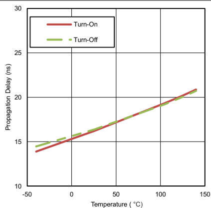
图 6-14. Input-to-Output Propagation Delay vs Temperature
