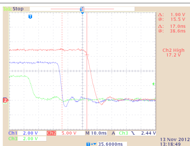
图 8-3. UCC27531DBV Input vs Output PWM Propagation Delay (low)
