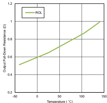
图 6-12. Output Pulldown Resistance vs Temperature
