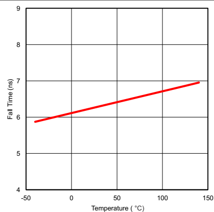
图 6-16. Fall Time vs Temperature
