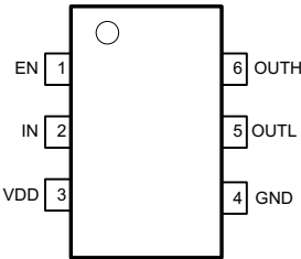
图 5-1. DBV Package 6-Pin SOT-23 Top View
