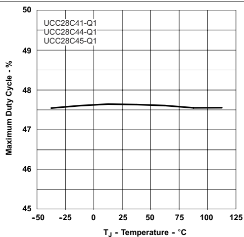
图 7-17. Maximum Duty Cycle vs Temperature
