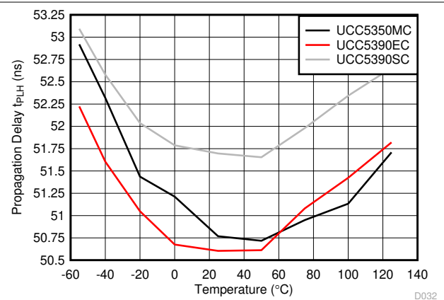
图 6-32. Propagation Delay t_{PLH} vs Temperature
