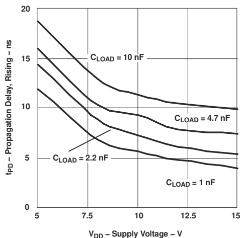
图 8-9. Propagation Delay Rising vs Supply Voltage
