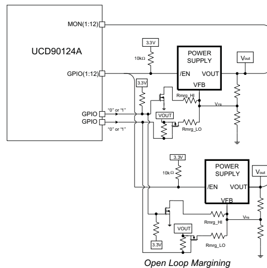
Figure 23. Open-Loop Margining
