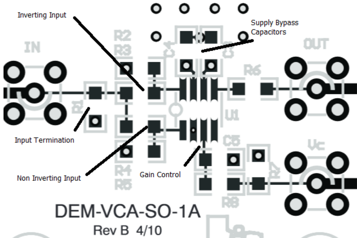
Figure 49. Layout Example
