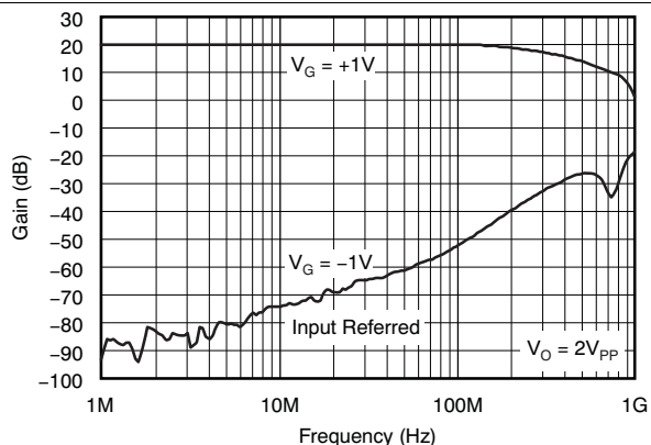
Figure 39. Fully-Attenuated Response
