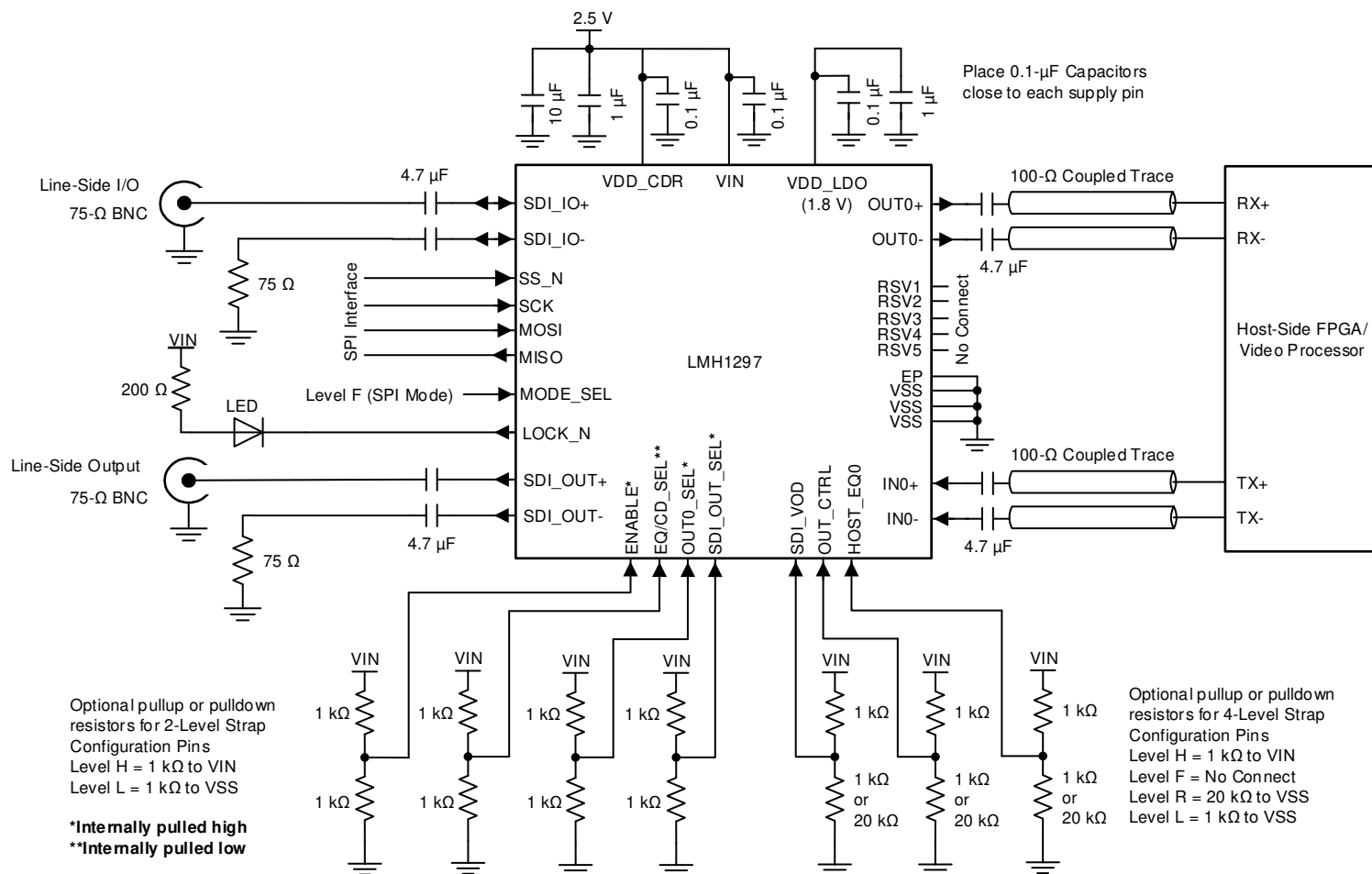
图 9-1. LMH1297 Typical Application Circuit
