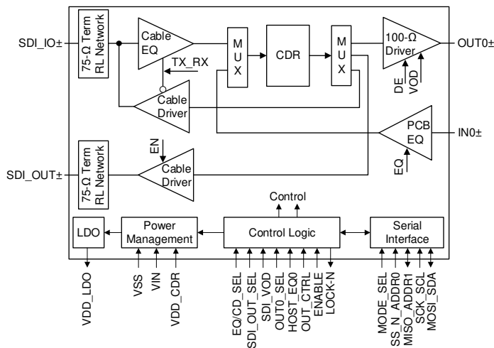
图 8-1. LMH1297 Block Diagram Overview
