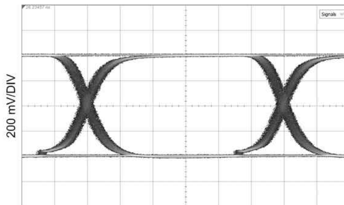
图 9-21. 270 Mbps, CC = 600-m Belden 1694A, Reclocked
