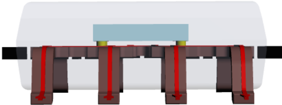
Device side view
