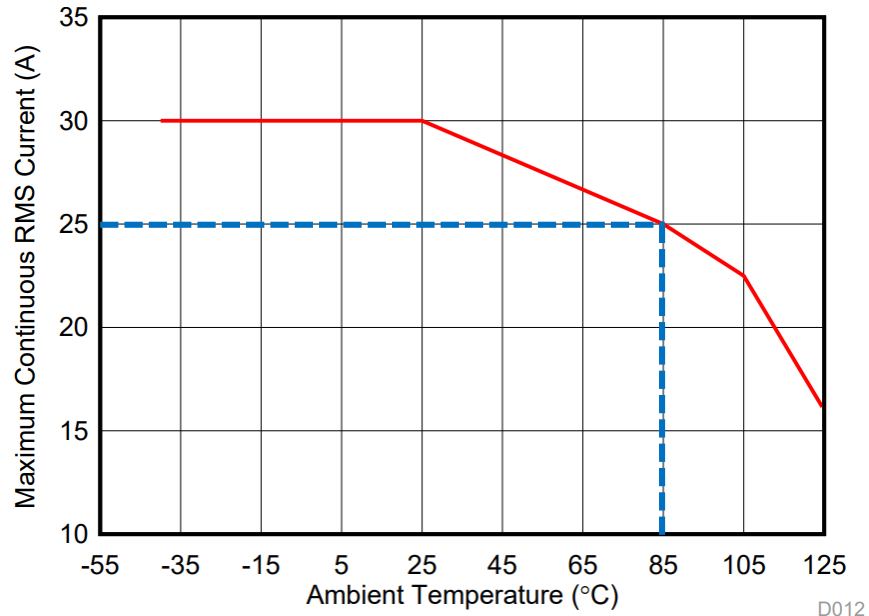
Example continuous current capability
