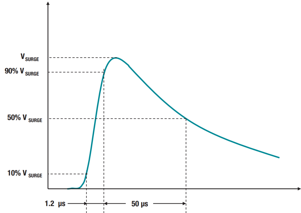
Surge impulse test profile
