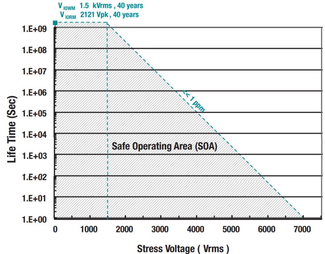
Example TDDDB plot
