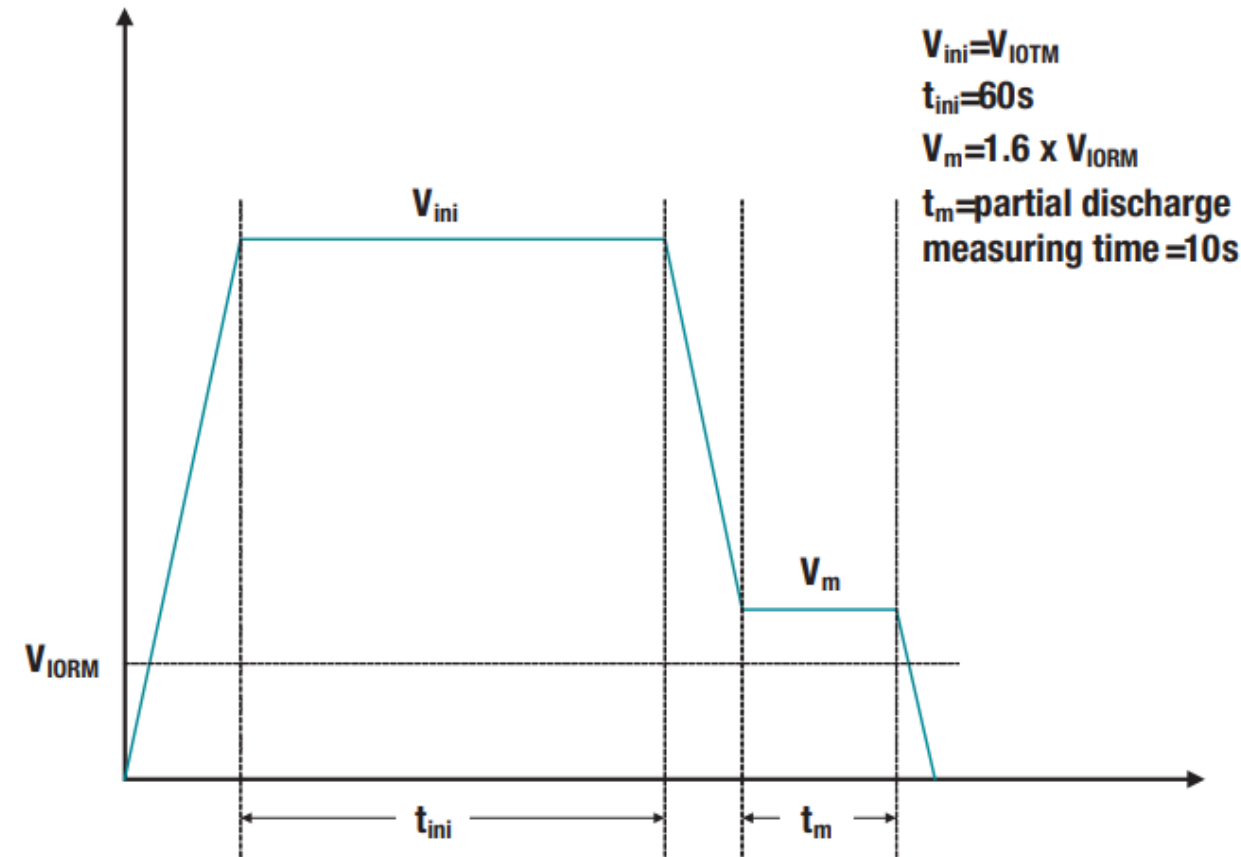
Simplified Method A test profile
