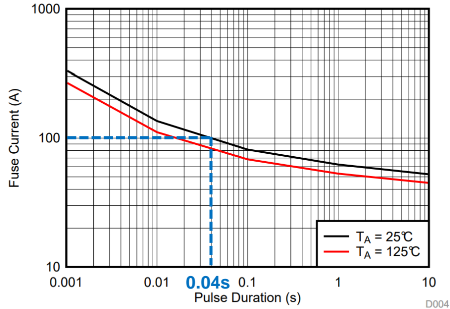
Example pulse current capability
