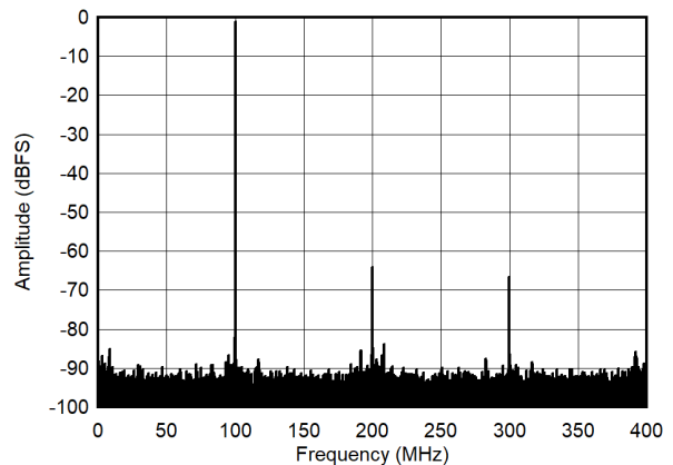
Low Power Mode Figure 5-10. Single Tone FFT at 100MHz and -1dBFS
