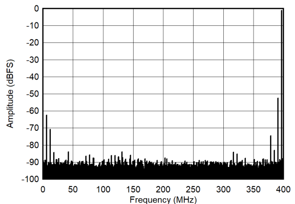
Low Power Mode Figure 5-12. Single Tone FFT at 1197MHz and -1dBFS
