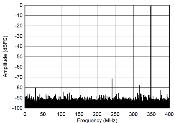
Low Power Mode Figure 5-11. Single Tone FFT at 347MHz and -1dBFS
