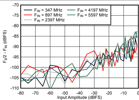
Figure 6-75. Dual Channel Mode: F_S/2 - F_{IN} vs Input Amplitude and Frequency
