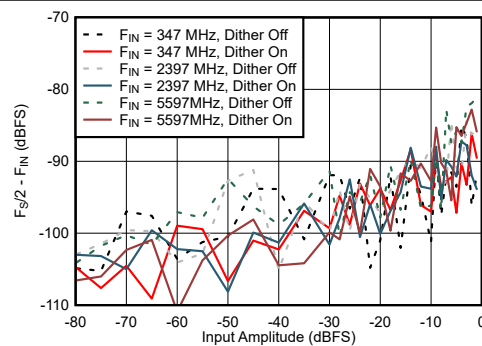
Figure 6-76. Dual Channel Mode: F_S/2 - F_{IN} vs Input Amplitude and Dither
