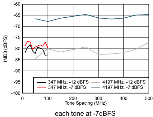
Figure 6-109. Dual Channel Mode: IMD3 vs Tone Spacing
