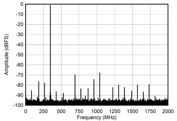
Figure 8-3. FFT for 347 MHz Input Signal, 4 GSPS, JMODE3
