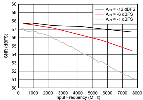
Figure 6-82. DES Mode: F_{IN} \pm F_S/4 vs Input Frequency
