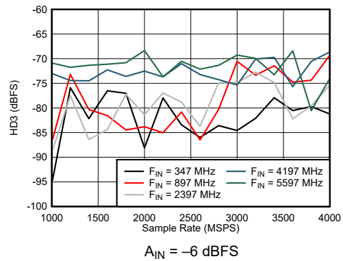
Figure 6-52. Dual Channel Mode: HD3 vs Sample Rate and Input Frequency
