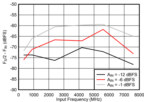
Figure 6-81. DES Mode: F_S/2 - F_{IN} vs Input Frequency
