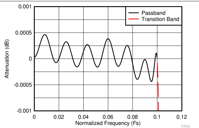
Figure 7-12. Decimate-by-4 Composite Zoomed Pass-Band Response
