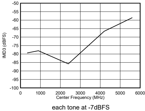
Figure 6-105. Dual Channel Mode: IMD3 vs Input Frequency
