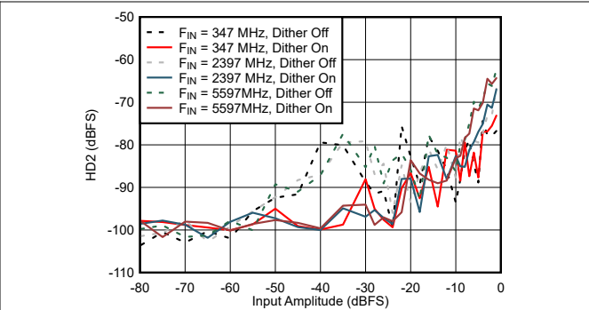
Figure 6-60. DES Mode: HD2 vs Input Amplitude and Dither
