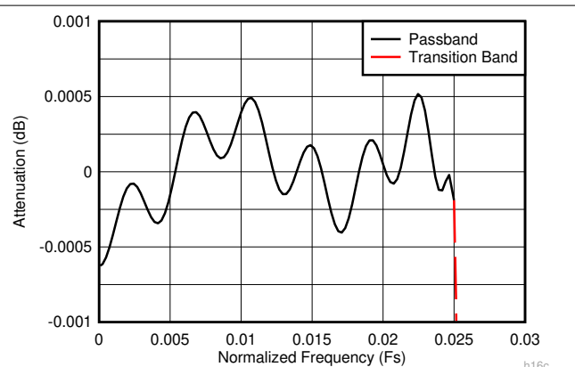
Figure 7-16. Decimate-by-16 Composite Zoomed Pass-Band Response
