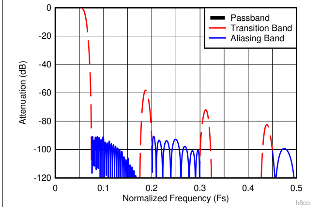
Figure 7-13. Decimate-by-8 Composite Response
