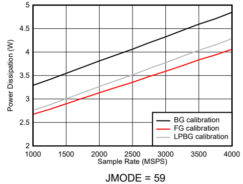
Figure 6-135. Dual Channel Mode: Power Dissipation vs Sample Rate
