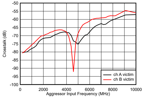
Figure 6-5. Crosstalk vs Input Frequency
