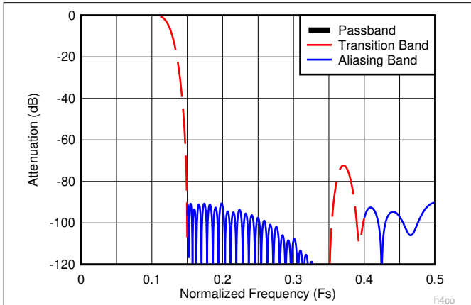
Figure 7-11. Decimate-by-4 Composite Response
