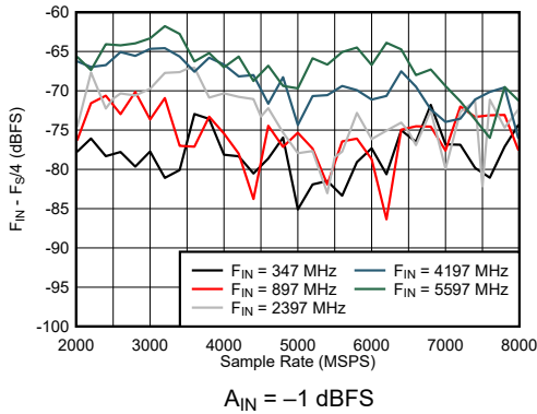
Figure 6-41. DES Mode: F_{IN} \pm F_S/4 vs Sample Rate and Input Frequency
