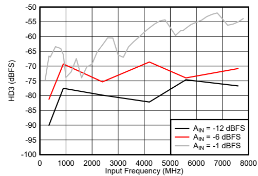
Figure 6-86. Dual Channel Mode: HD3 vs Input Frequency
