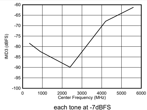
Figure 6-104. DES Mode: IMD3 vs Input Frequency
