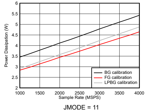
Figure 6-133. Dual Channel Mode: Power Dissipation vs Sample Rate
