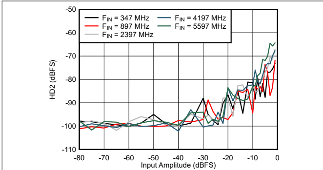
Figure 6-59. DES Mode: HD2 vs Input Amplitude and Frequency
