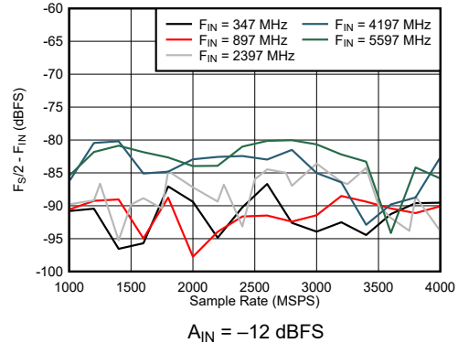
Figure 6-54. Dual Channel Mode: F_S/2 - F_{IN} vs Sample Rate and Input Frequency
