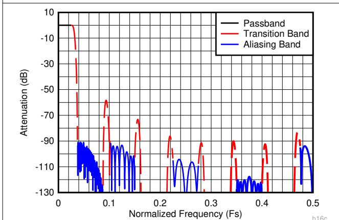
Figure 7-15. Decimate-by-16 Composite Response
