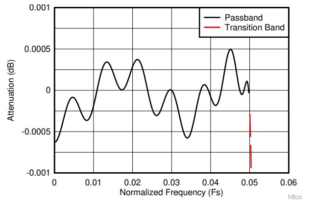
Figure 7-14. Decimate-by-8 Composite Zoomed Pass-Band Response
